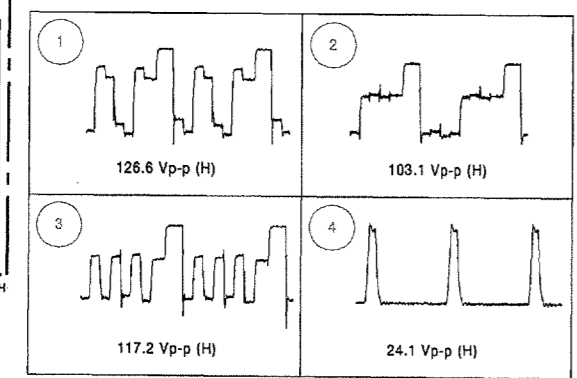
C BOARD WAVEFORMS
